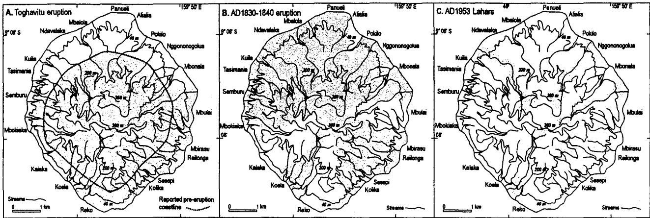
Fig. 4 Areas (stippled) affected by eruptions as described in Kastom legends from Savo as collected by Toba (1993). A Toghavitu event; unstippled area in the north represents the
