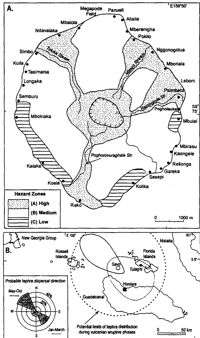
Fig. II Simple volcanic hazard assessment maps for Savo. A Flow hazards on Savo, particularly BAFs, ash-cloud surges and lahars, divided into three zones. B Tephra fall hazards estimated from a 0.1 \text{ km}^3 eruption of Savo at two different times of the year, adapted from Latter (1991). Inset: wind rose diagram of surface wind directions from Hydrographer of the Navy (1988)
